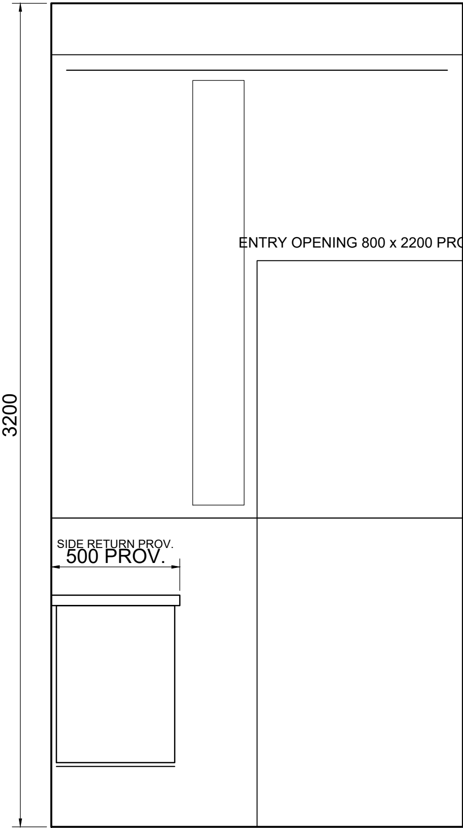
WASH SIDE ELEVATION
