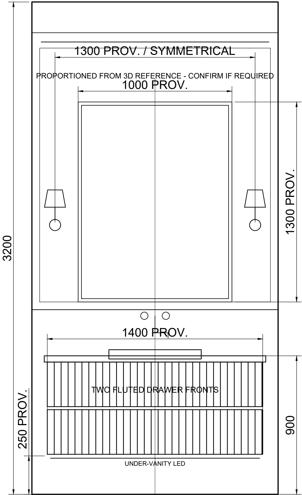
MAIN VANITY / MIRROR ELEVATION
