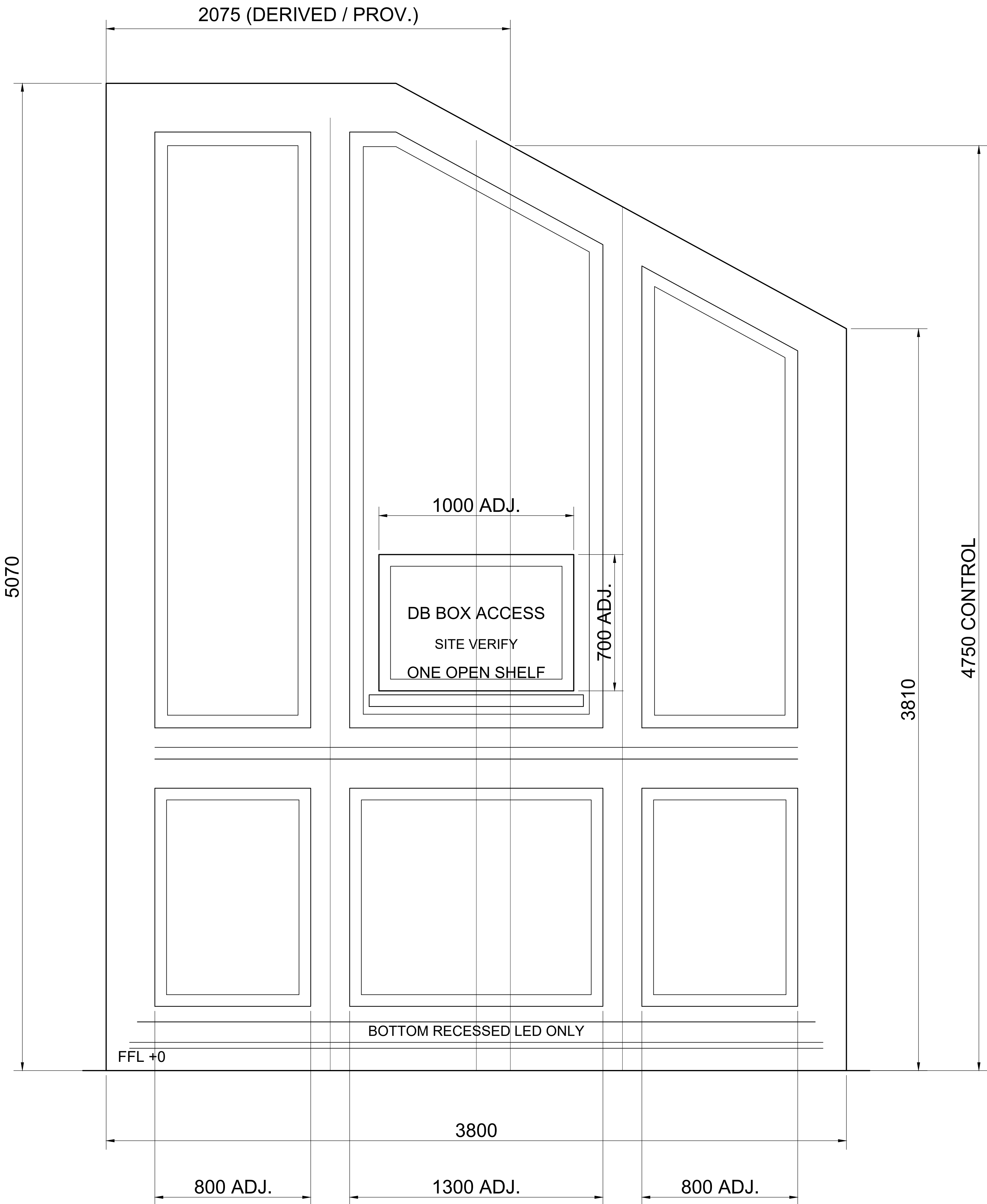
FRONT ELEVATION - STAIR WALL
